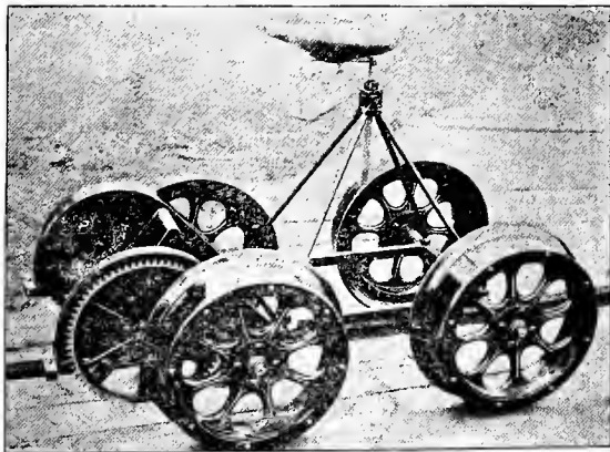
Fig. 5618. MINE AND TUNNEL VELOCIPEDE-CAR. SHEFFIELD CAR COMPANY, THREE RIVERS, MICHIGAN.
